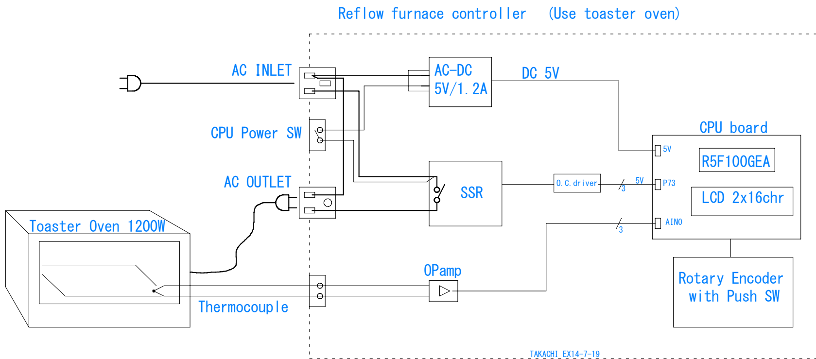
Connection diagram
